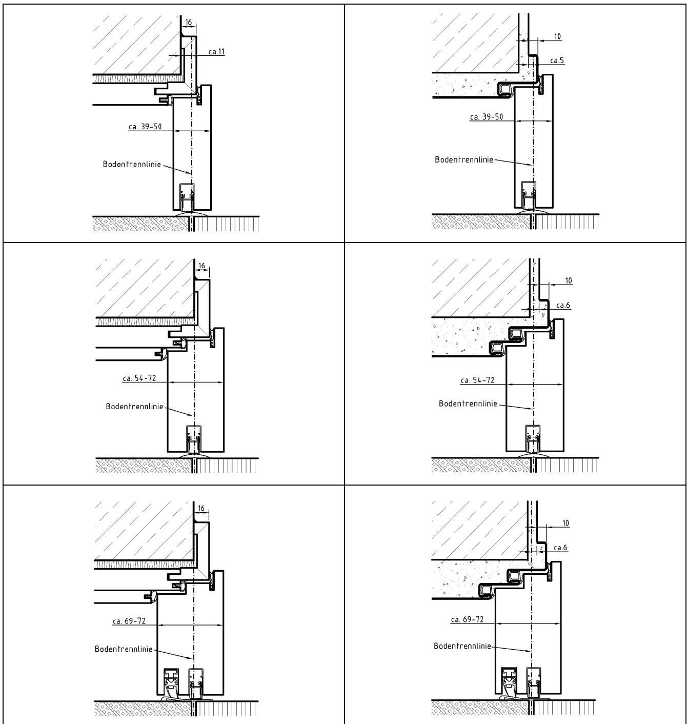
Holzzarge
